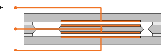
Fig. 2 : Cross section of a Colibrys accelerometer
