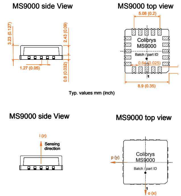
Fig. 6 : MS9000 LCC20 packaging
